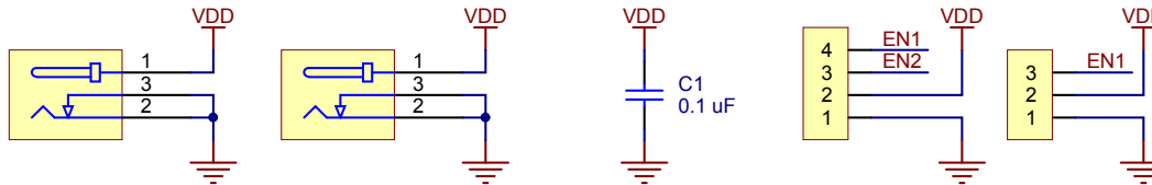
DC barrel jacks (center-positive)
