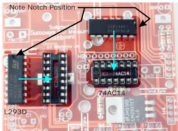
Step 6: Installing L293 and 74AC14 into carriers
