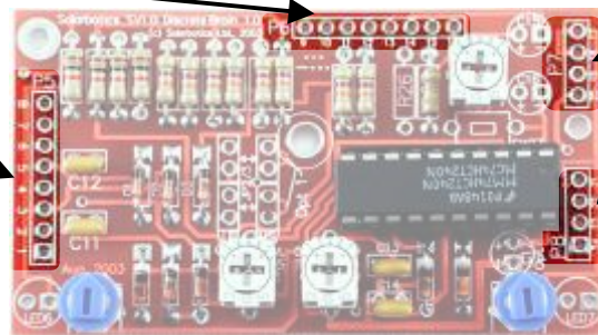
Steps 46 & 47: 8 and 4 pin installation UNDERNEATH!
