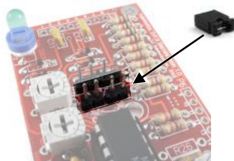
Step D: Install the jumpers on the pin pair on the 'MS' side (right side)
