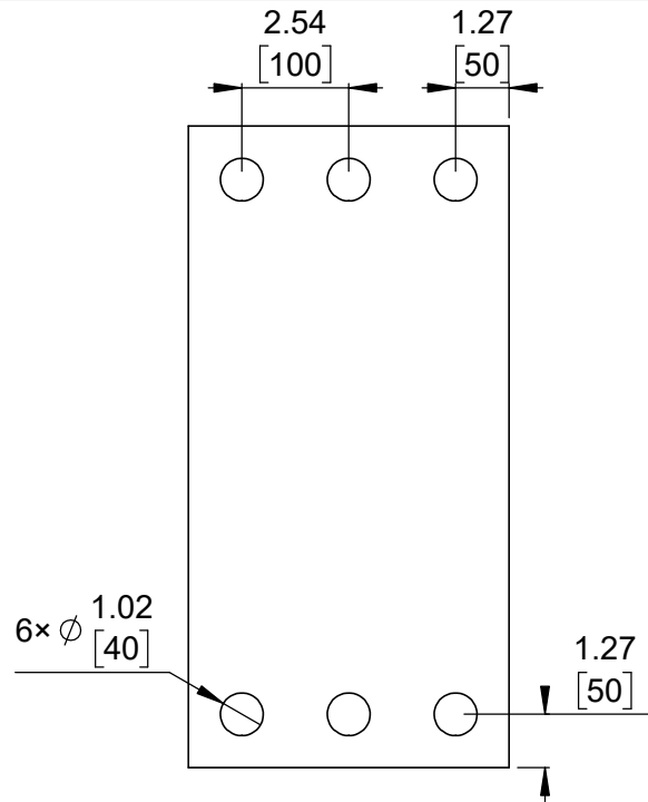
② Connector callouts (bottom view) Scale 5:1
