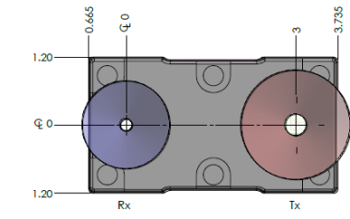
Figure 21. Outline drawing (5/5)
