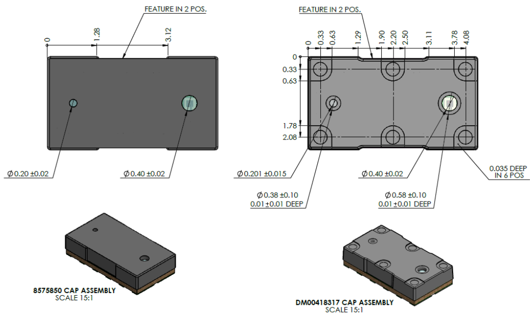
Figure 18. Outline drawing (2/5)
