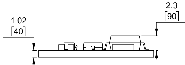
④ Profile, no connectors Scale 3:1
