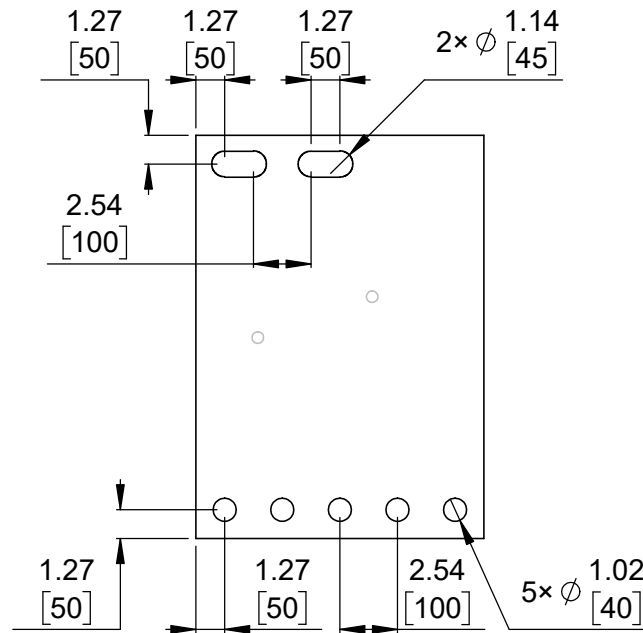
② Connector callouts (bottom view) Scale 3:1
