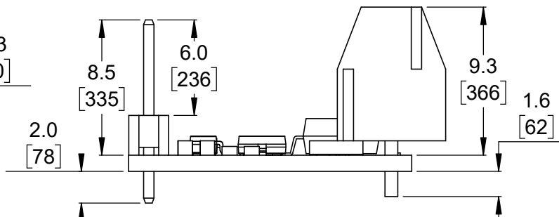
⑤ Profile, soldered connectors Scale 3:1
