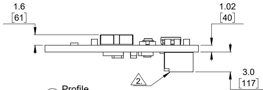
④ Profile Scale 3:1
