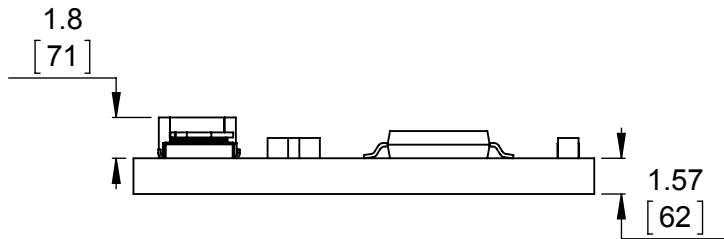
4 Profile Scale 3:1
